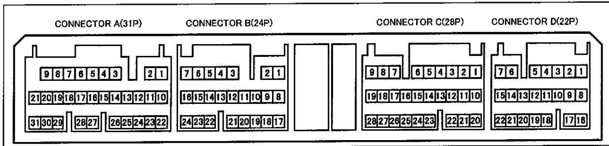
e-manage Ultimate Wire Diagram
