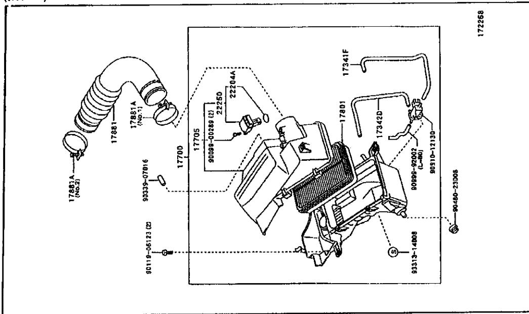
Fig. 1703/ Air Cleaner (8908- )
