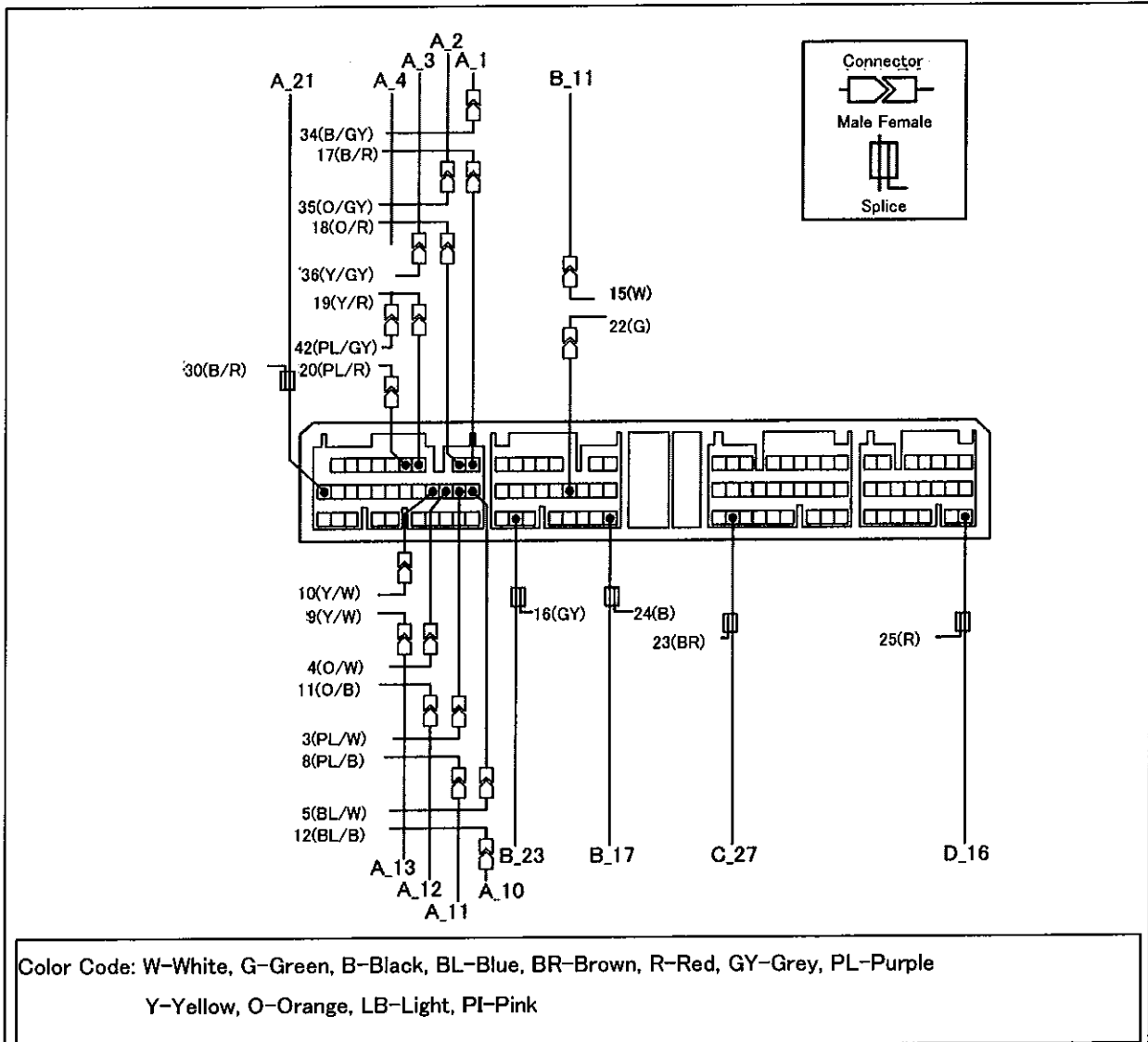
e-manage Ultimate Wire Diagram
