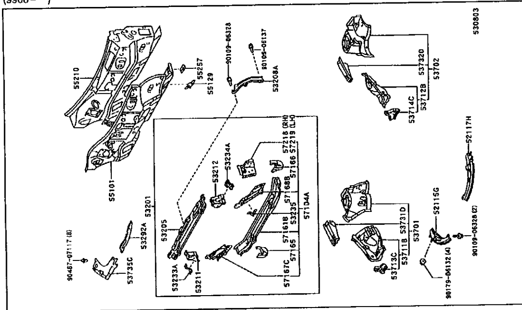
Fig. 5304/ Front Fender Apron & Dash Panel (9908- )
